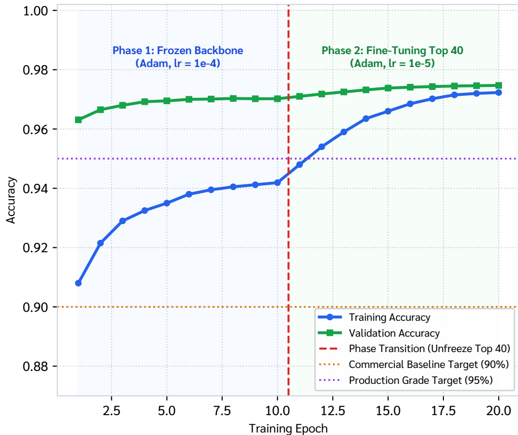
Figure 3(a): Model Classification Accuracy Across Training Epochs (Evaluating Convergence Against Commercial Thresholds)
