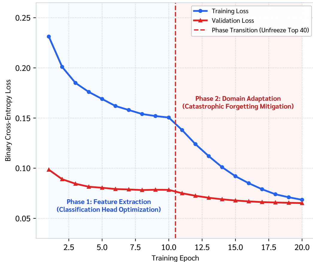
Figure 3(b): Binary Cross-Entropy Loss Convergence (Verifying Two-Phase Loss Decay Stability)
